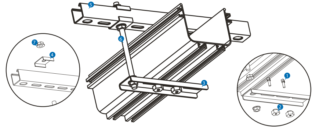
STRUT CHANNEL MOUNTING SUPPORT (SUIT FOR ALL THE SIZES)
