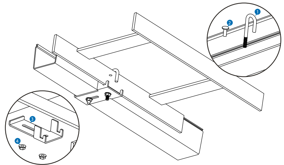
60x60 LADDER RACK MOUNTING
