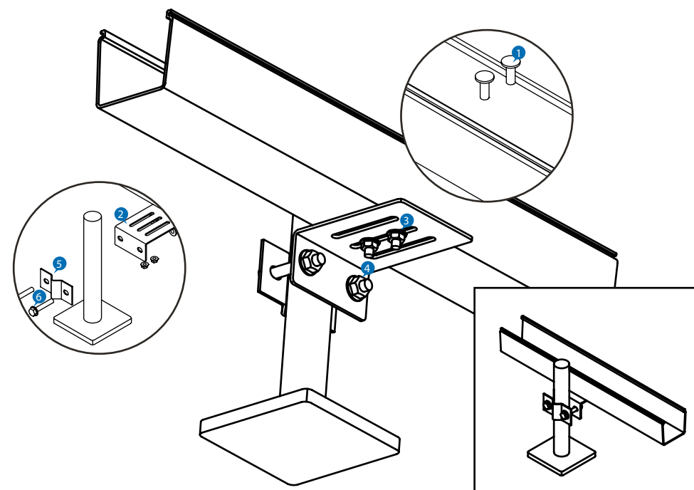
60x60 UNDER ACCES FLOOR MOUNTING
