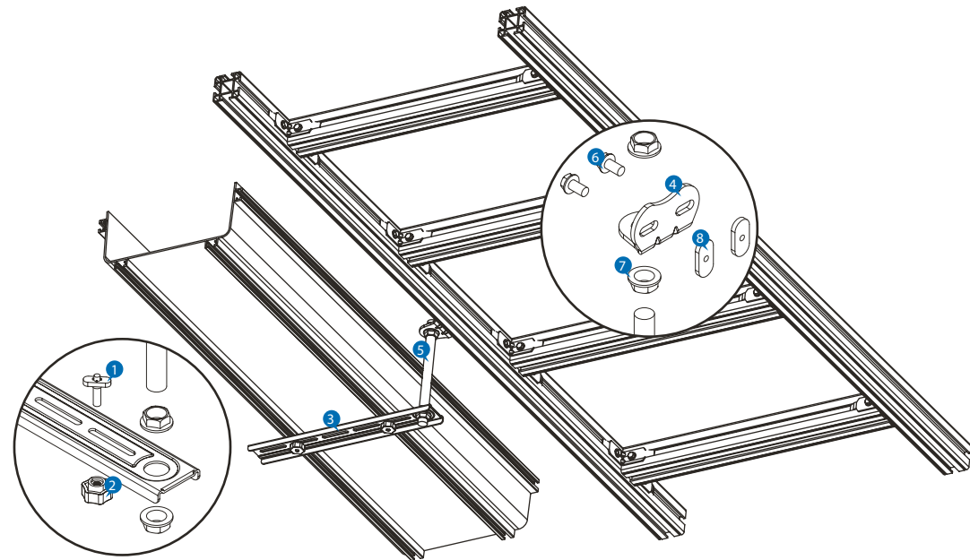
ALUMINUM LADDER RACK SIDE SUPPORT (SUIT FOR ALL THE SIZES)
