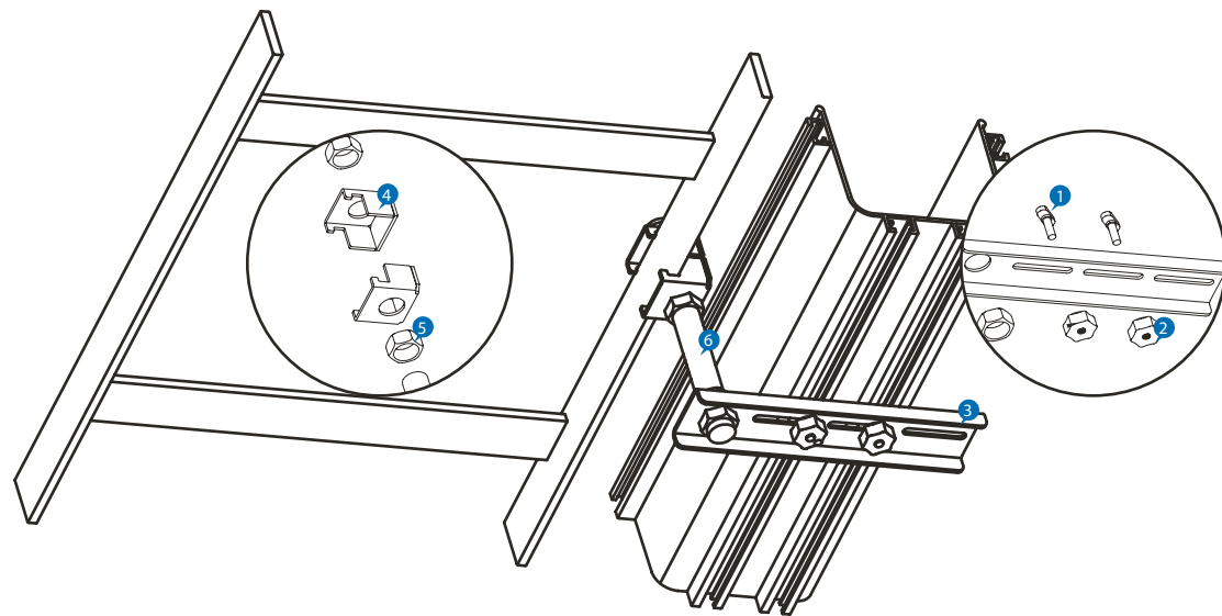
FLAT STEEL LADDER RACK SIDE SUPPORT (SUIT FOR ALL THE SIZES)
